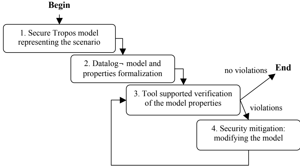
Figure 3: The analysis process using Secure Tropos.
