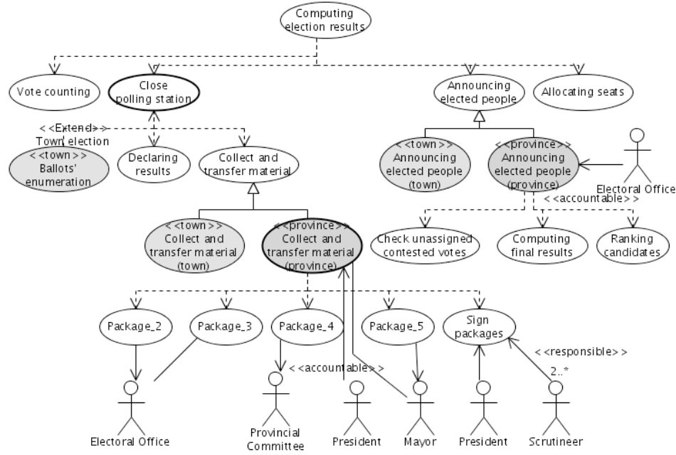
Figure 4: The UML as-is use case diagram
