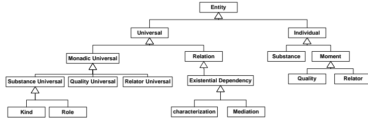
Figure 9. Excerpt of the Foundational ontology UFO-A.
